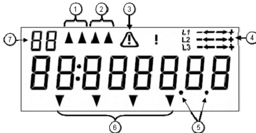
Figur 6. E120GiME-display
